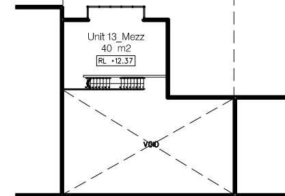
MEZZANINE LEVEL
